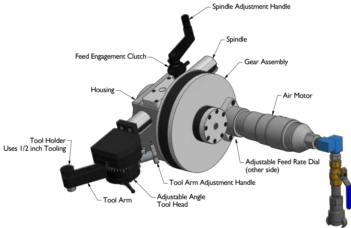
Mactech 624 Flange Facer
