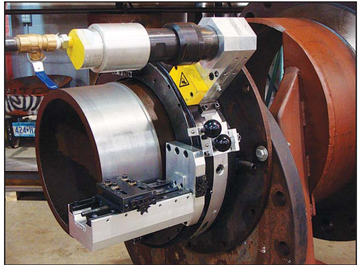
814LC Clamshell with Axial Feed Accessory
