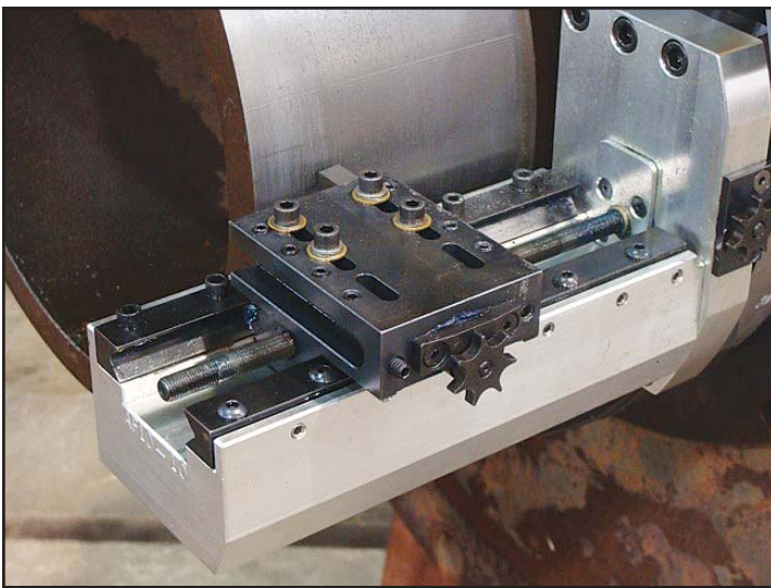
Axial Feed Accessory Machining Pipe
