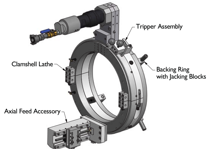
Axial Feed Accessory and Backing Ring
