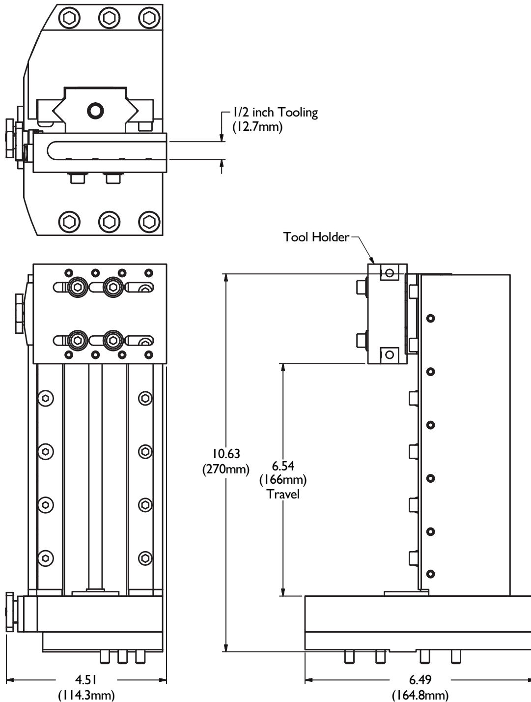
Axial Feed Accessory Dimensions
