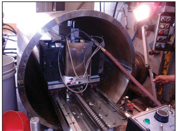
Keyway Cutting Long Tube
