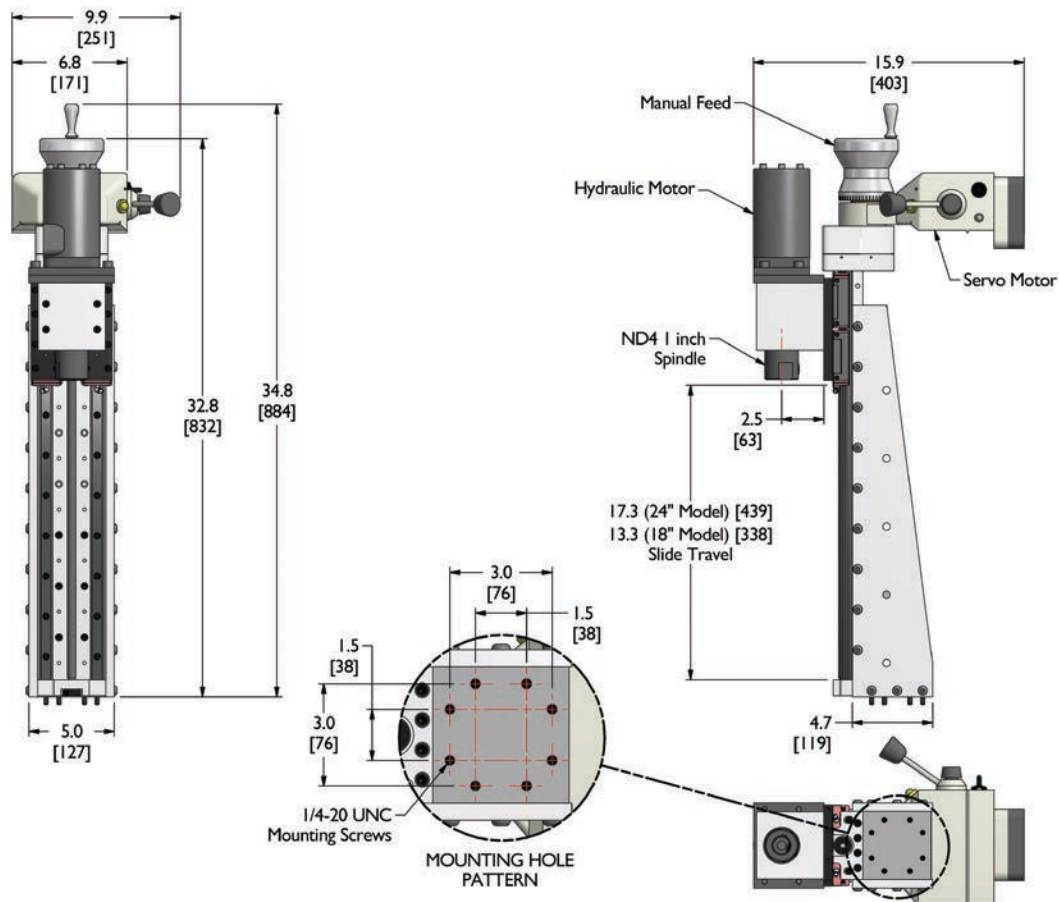
MT4 LRA Boring Mill
