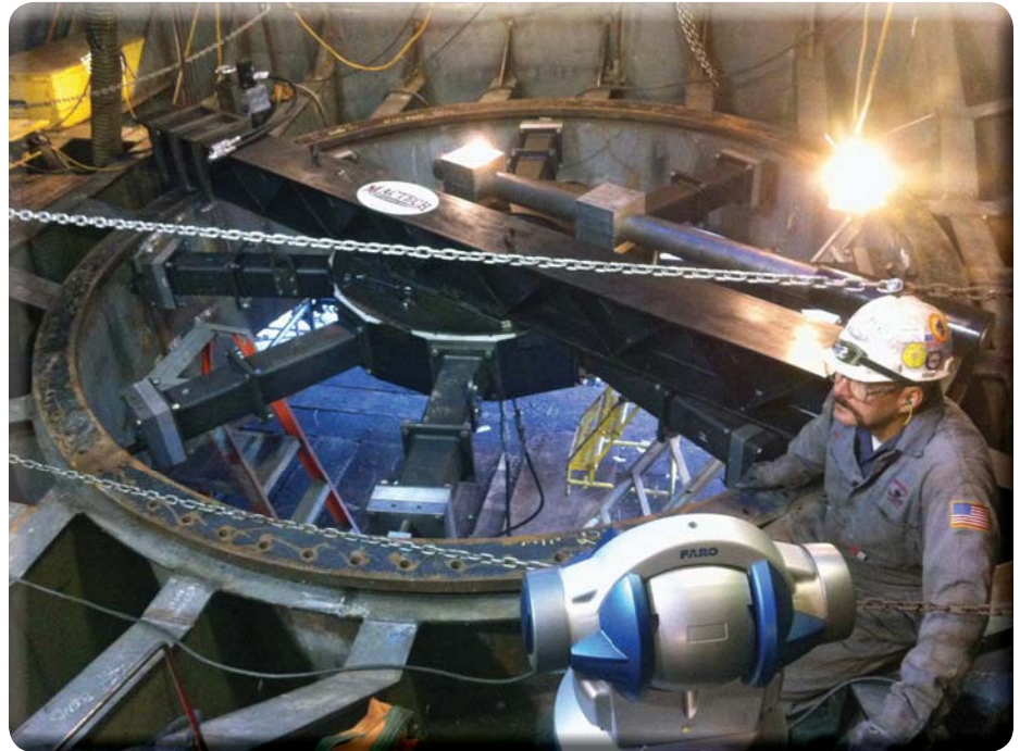
Large Diameter Facing with Laser Measurement
