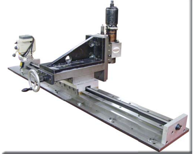
MT8 Portable Mill
