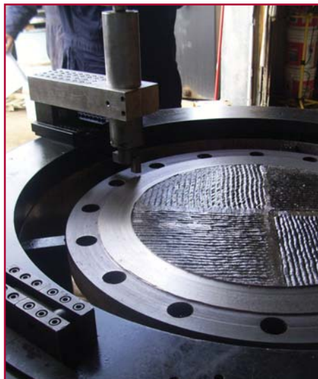
Flange Facing
